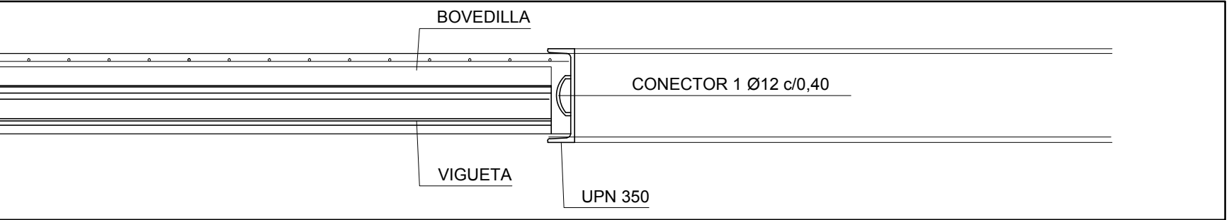
DETALLE 2-2
