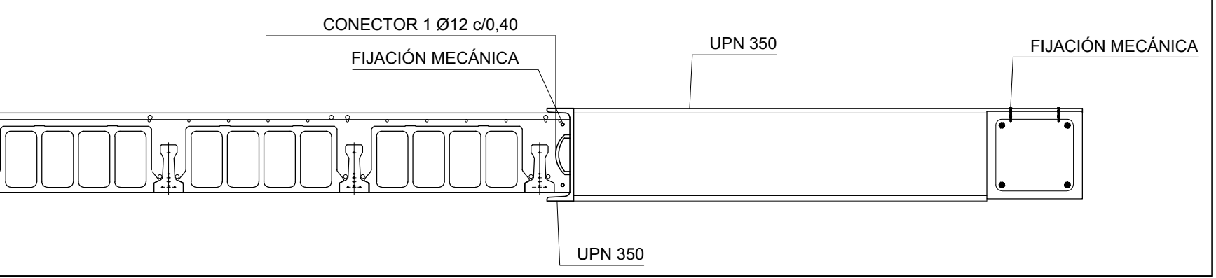
DETALLE 3-3
